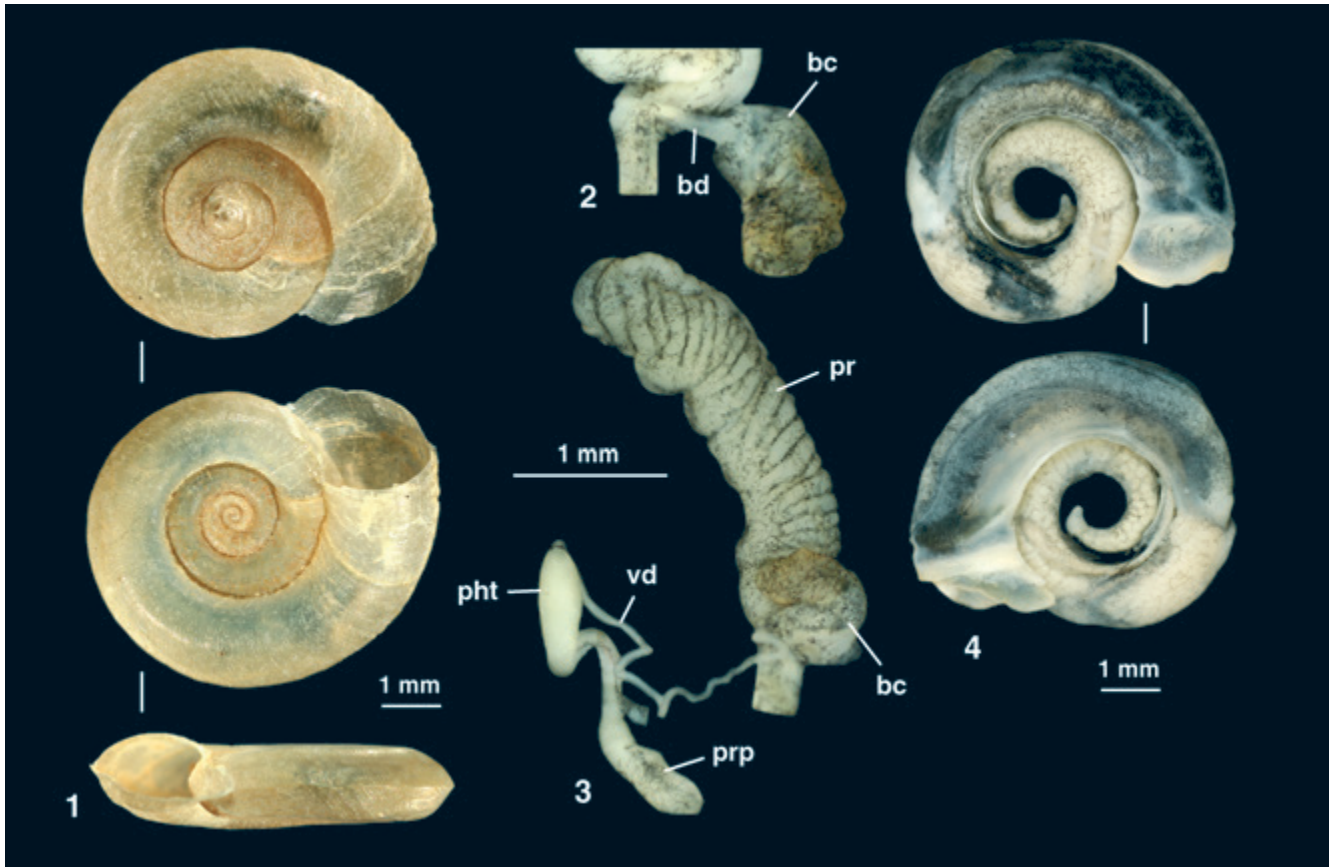
Fig. 4 Gyraulus acronicus , River Pang, Pangbourne Berkshire, England (11.07.2001 leg. I. Killeen). 1: Shell, 2: Bursa copulatrix, 3: Copulatory organs, 4: Mantle pigmentation. – bc = bursa copulatrix, bd = bursa duct, pht = phallosome, pr = prostata, prp = preputium, vd = vas deferens.
