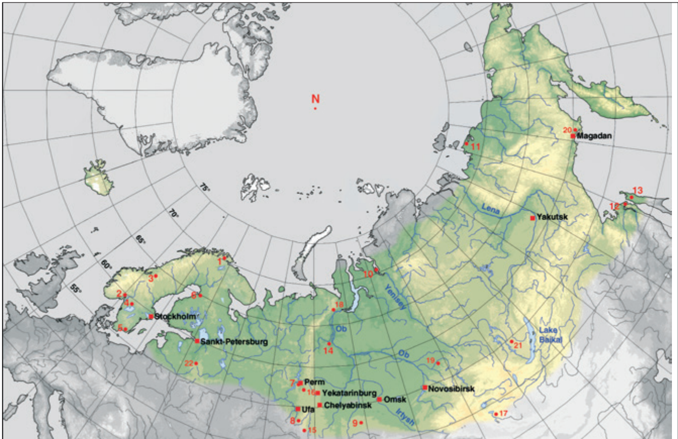
Fig. 5 The distribution of Gyraulus stroemi (Westerlund, 1881) in Eurasia. – Norway: 1: Östfinmarken (Johansen 1904), 2: Borrevatn, Vestfold (Økland 1990), Sweden: 3: Kall, Jämtland, 4: Karlstad, 5: Ronneby, Finland: 6: Oulu (Westerlund 1884: 51), Estonia: Wagula-See near Werro, Russia and Mongolia: 7: Perm, 8: Zlatoustovskaja, Orenburg, 9: Kazakhstan, Akmola region, 10: Jenissej (Johansen 1904), 11: Jana-Gebiet, 12: Nikolajewsk-na-Amure, 13: Sakhalin, 14: Beresowo town, 15: Gubernlinskaja, 16: Kljuchi, 17: Mongolia, Khovd Aimak, 18: Tyumen Region, Vylposl channel in the Ob' River floodplain near Labytnangi, 19: Tomsk Region, waterbodies of the Chulym River near Tegul'det Settl, 20: Magadan, 21: Bulga River, 22: Seliger Lake. - Type locality (blue circle): Ekker in Rökkebjergstjern (Norway).
