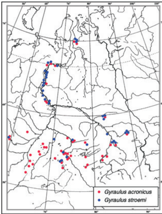
Fig. 7 The distribution of G. acronicus and G. stroemi in W-Siberia. The map is based on the electronic catalogue of the Museum of Siberian Aquatic Molluscs, Omsk.
